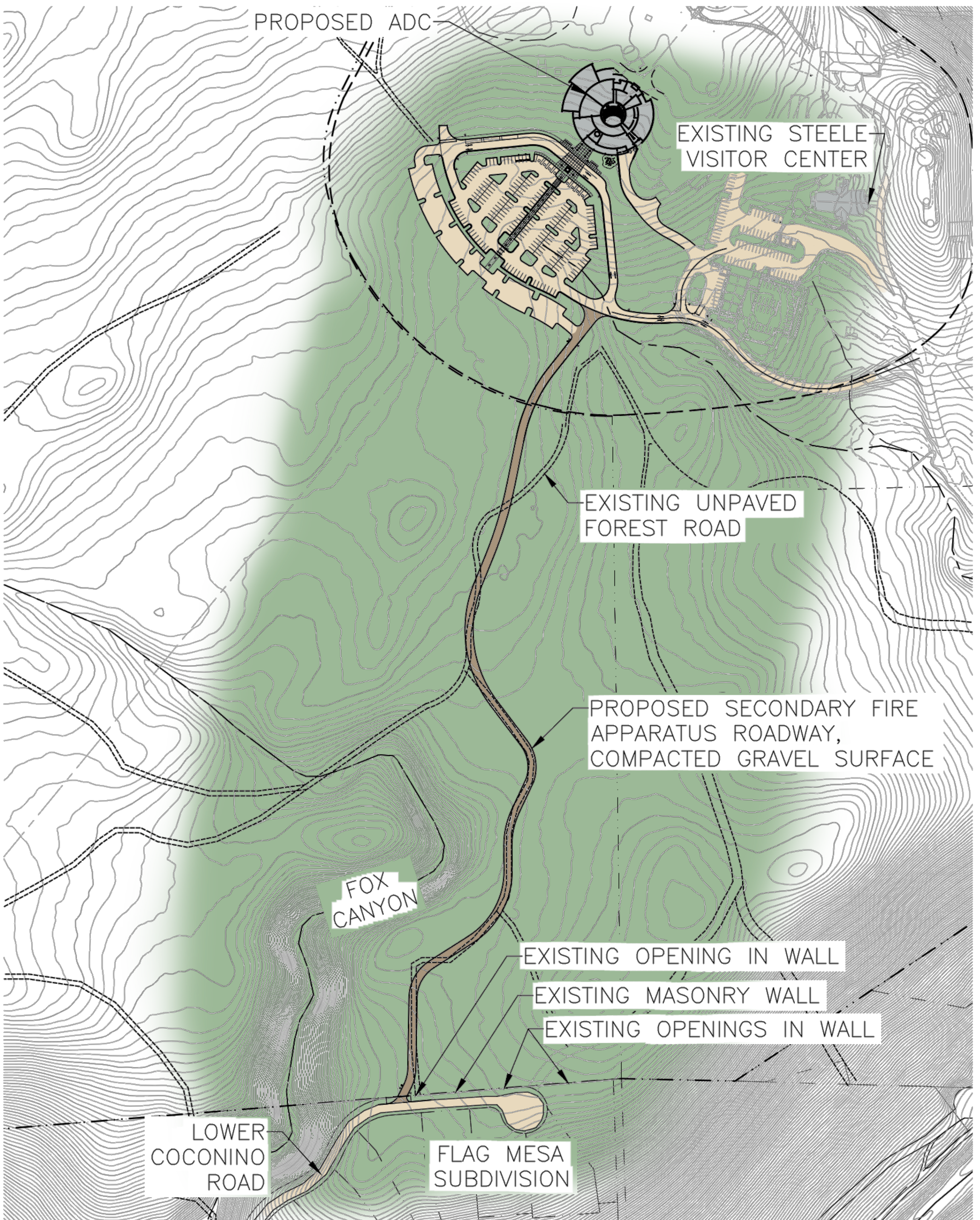
SECONDARY FIRE APPARATUS ACCESS ROADWAY (1)
